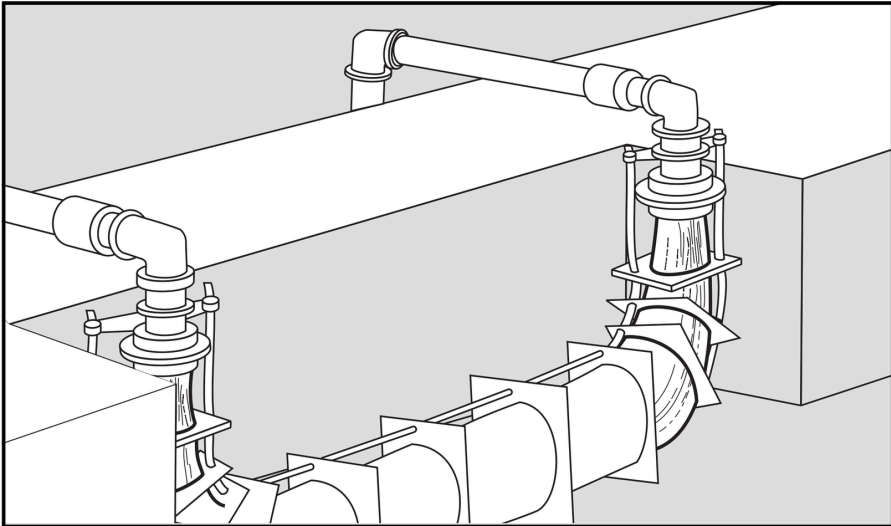
Figure 2 Install piers or pilasters at both ends of coils or create a protective cavity for the length of each coil.
